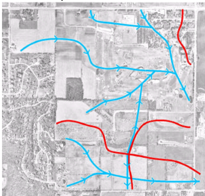
Exhibit 5: Primary stormwater sheds and flow lines
